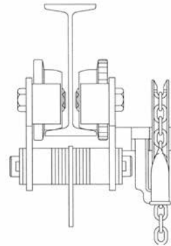
MODEL PT PLAIN TROLLEY
