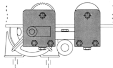
GEARED TROLLEY
