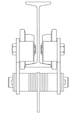
MODEL PT GEARED TROLLEY
